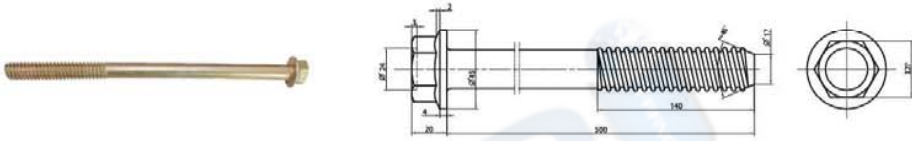
Square flange bolts with round thread for tunnel
